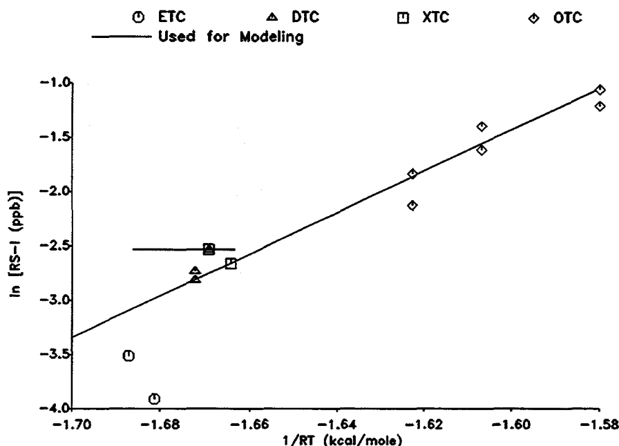
Figure 18. Arrhenius plot showing the temperature dependence of radical source input parameters which fit the ETC, DTC, XTC, and OTC n-butane runs.
