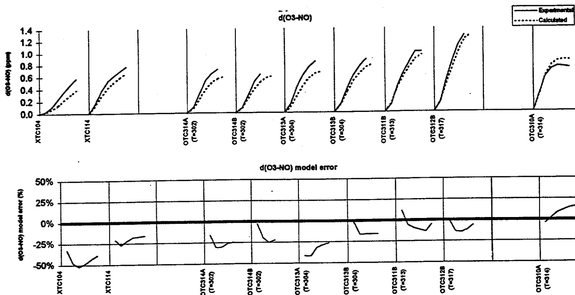
Figure 33. Results of model simulations of d(O_3-NO) in surrogate - NO_x experiments carried out in the XTC and the OTC. OTC high NO_x runs (middle set) are ordered by temperature.
