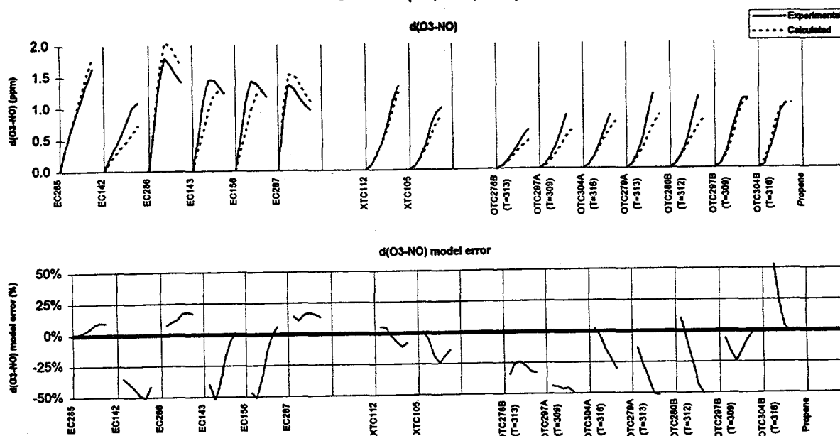
Figure 22. Results of model simulations of d(O_3-NO) in the ethene - NO_x experiment carried out in the xenon arc or outdoor chambers. Runs are ordered by ROG/NO_x .
