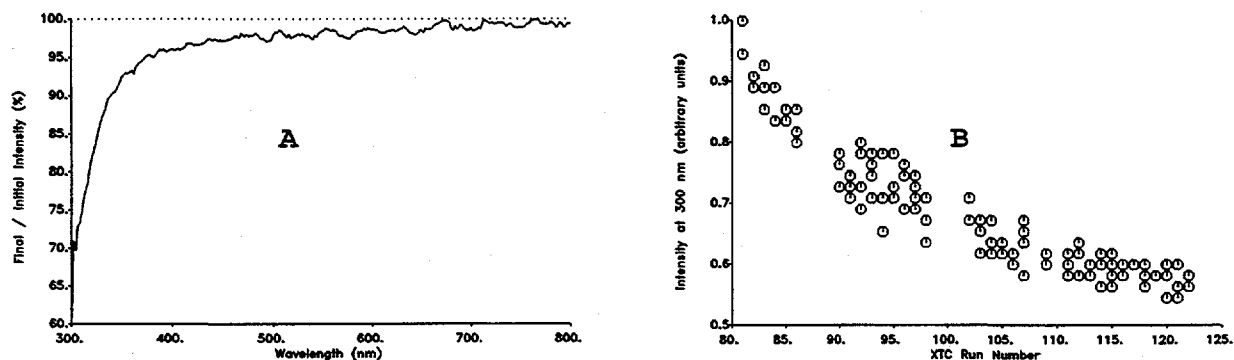
Figure 11. (A) Ratio of spectrum of run XTC120 relative to that of run XTC081 against wavelength, showing the decline of spectral intensity as a function of wavelength during the experiments for this program. (B) Plot of relative intensity at 300 nm against XTC run number.
