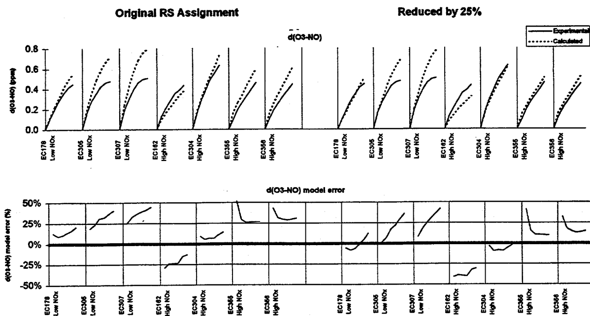
Figure 16. Results of model simulations of d(O_3-NO) in the EC n-butane - NO_x runs using the previous and the adjusted radical source assignments.
