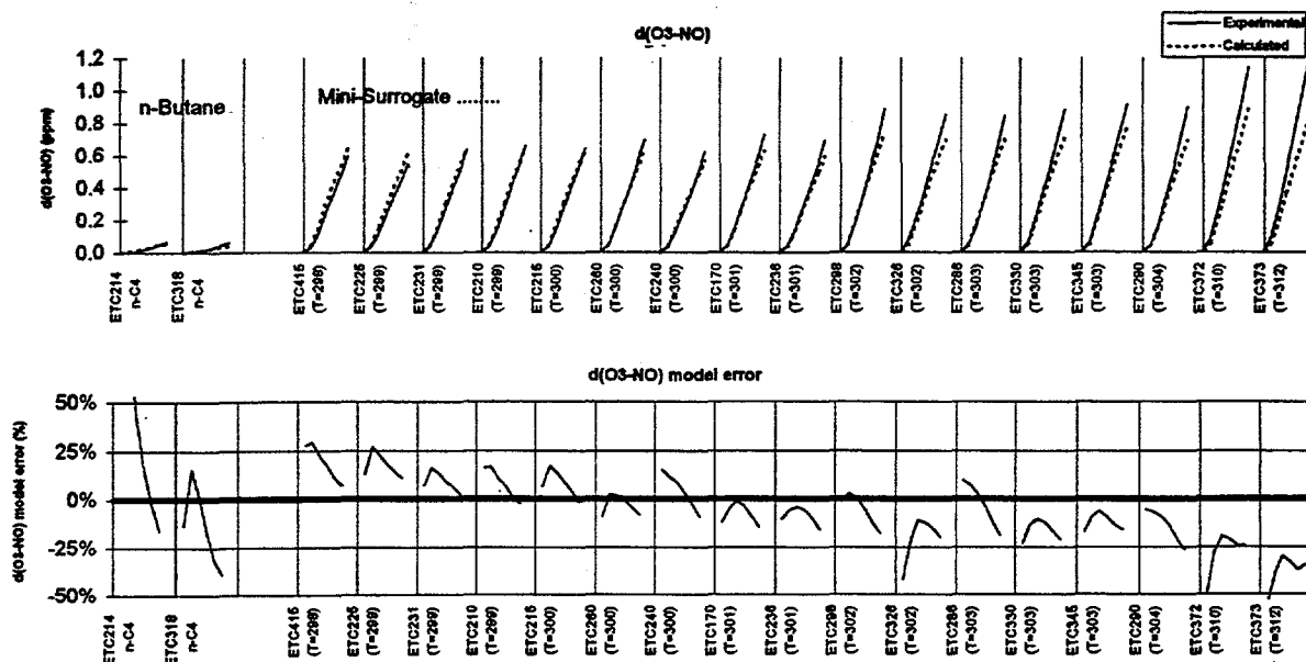
Figure 17. Results of model simulations of d(O_3-NO) in ETC n-butane - NO_x and in selected Set 3 mini-surrogate - NO_x experiments using the radical source assignment of Carter et. al (1993a). The mini-surrogate runs are ordered by temperature.
