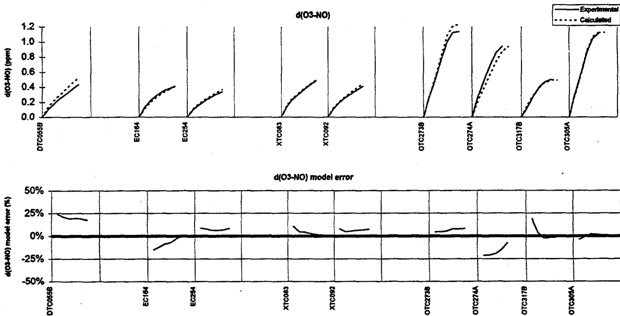
Figure 20. Results of model simulations of d(O 3 -NO) in the formaldehyde - NO x and the acetaldehyde - NO x experiments.
