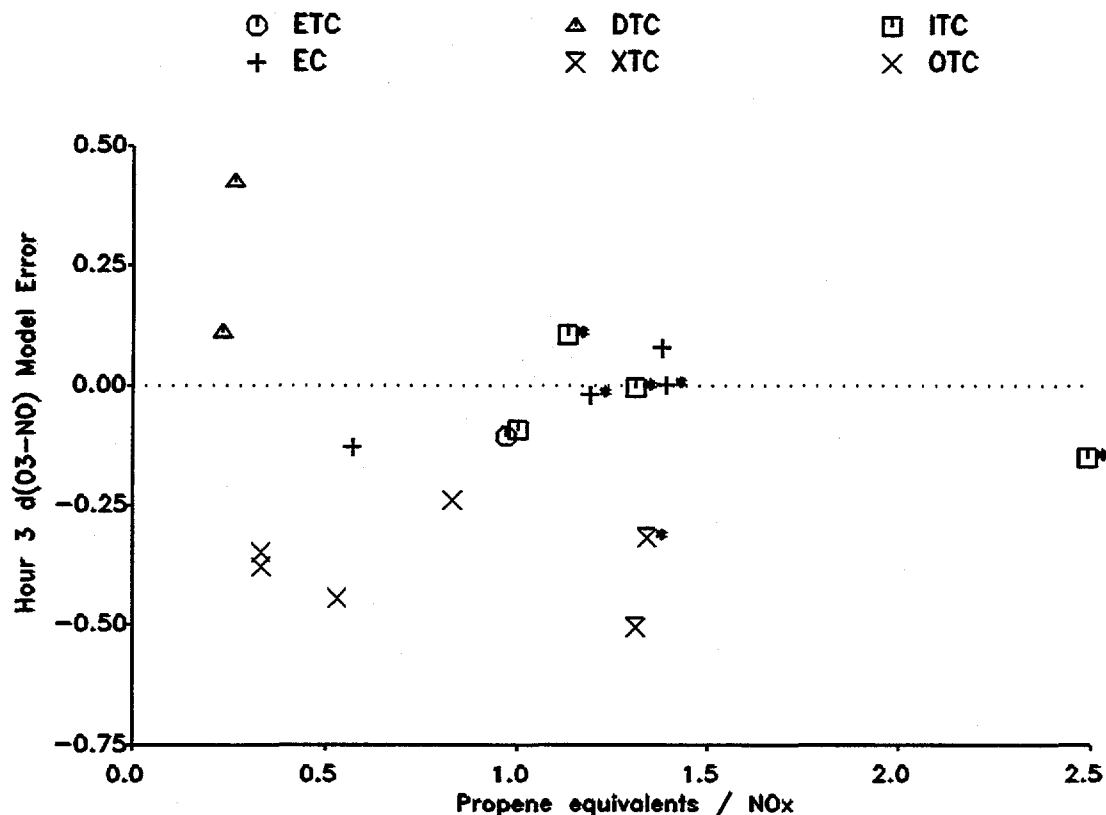
Figure 30. Plots of model bias for hour 3 d(O_3-NO) against initial ROG/NO x ratio for the m-xylene - NO x and 1,3,5-trimethylbenzene - NO x experiments. The 1,3,5-trimethylbenzene experiments are indicated with a "*" after the plot symbol.
