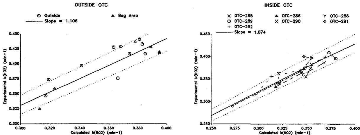
Figure 12. Plots of experimental vs calculated NO 2 photolysis rates measured in or around the Outside Teflon Chamber.
