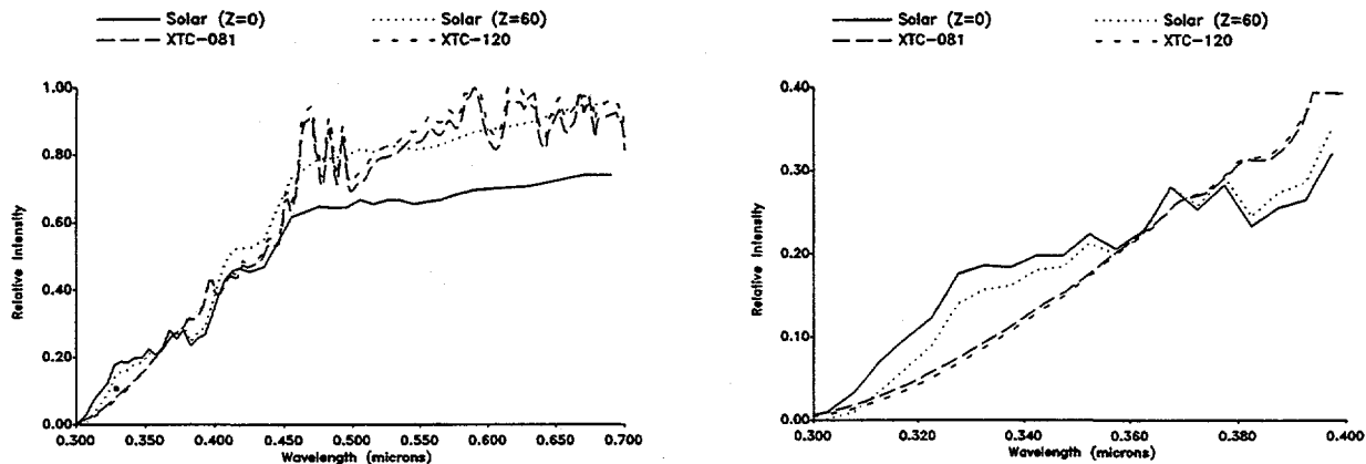
Figure 10. Representative XTC spectra compared with solar spectra for zenith angles of 0° and 60°. The spectra are all normalized to give the same NO 2 photolysis rate.
