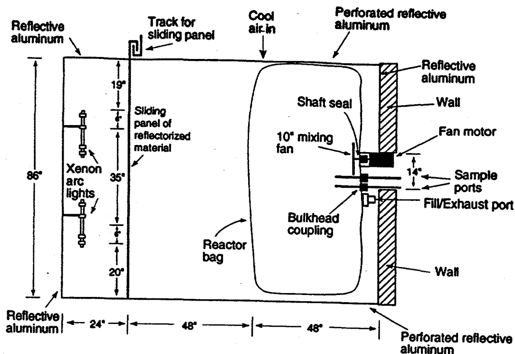
Figure 5. Side view of Xenon Teflon Chamber.
